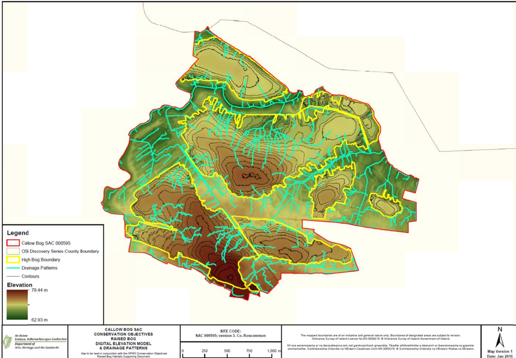
Map 3: Digital elevation model and drainage patterns at Callow Bog.
