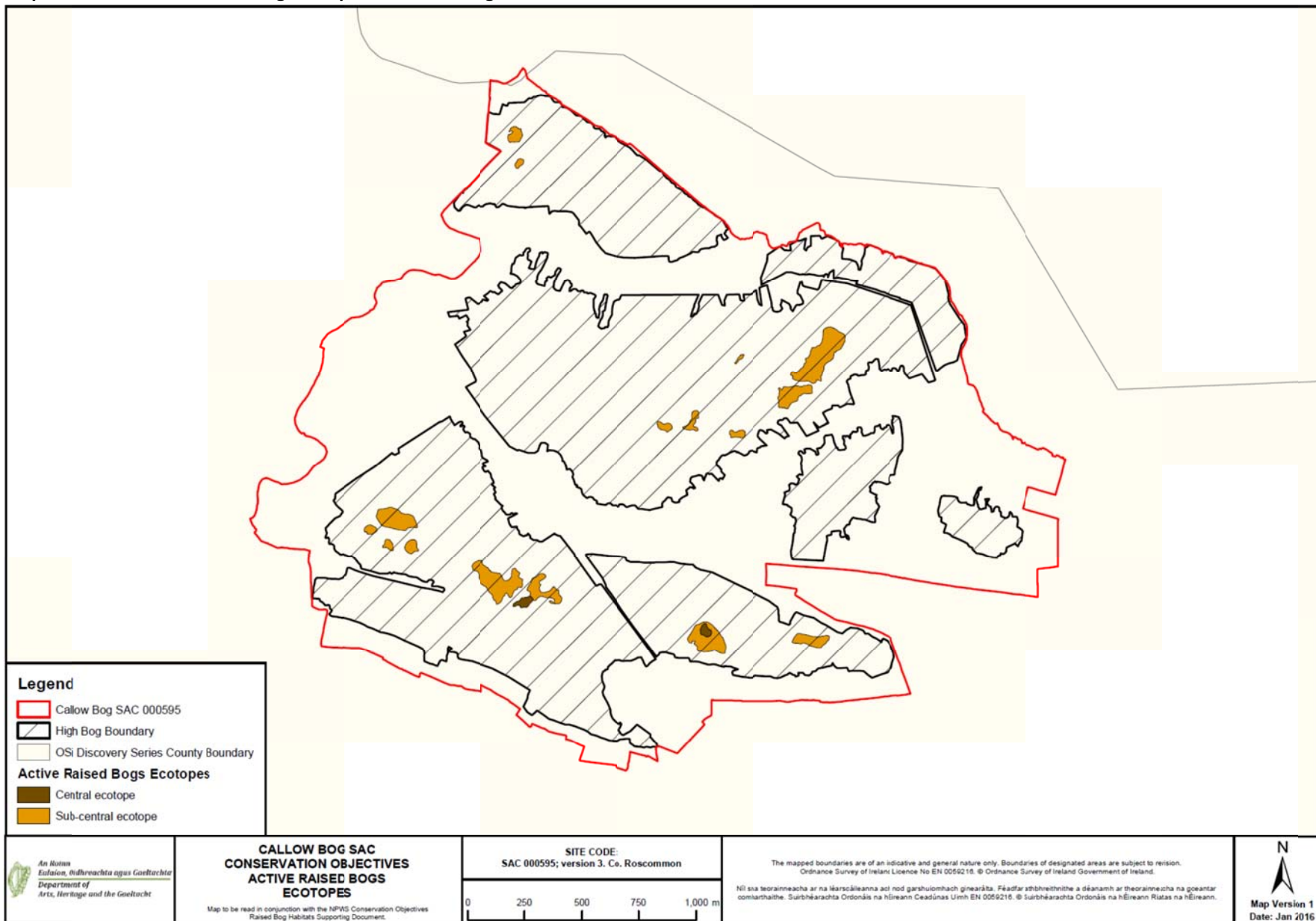
Map 2: Distribution of raised bog ecotopes on Callow Bog.
