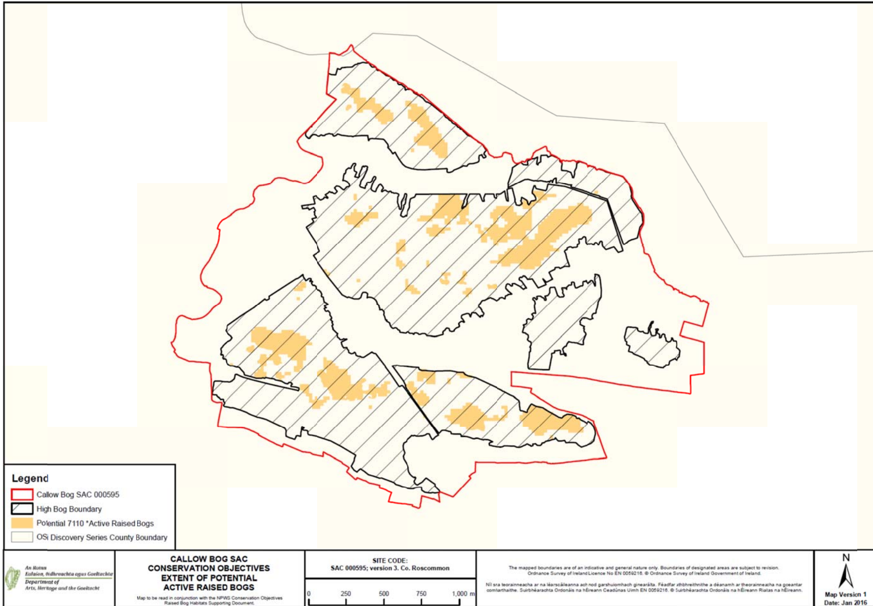
Map 1: Extent of potential active raised bog on Callow Bog.
