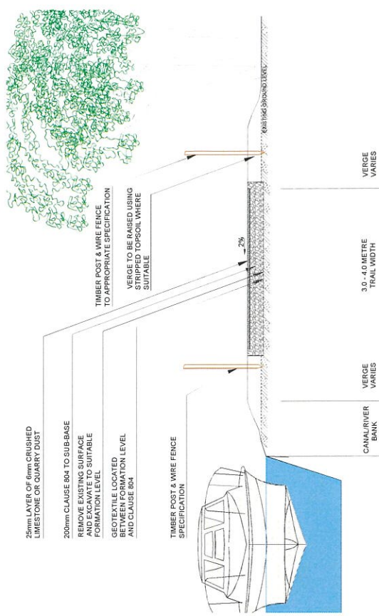
TYPICAL RECREATIONAL TRAIL CROSS-SECTION - UNBOUND (FENCED)
