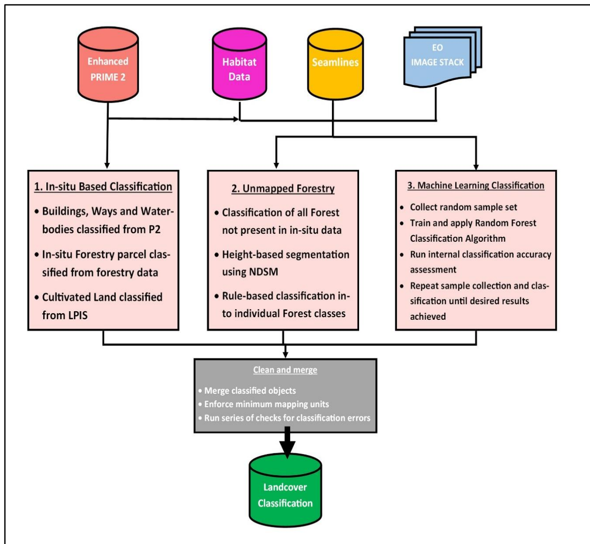
Figure 4.3: Diagram giving an overview of the classification workflow
