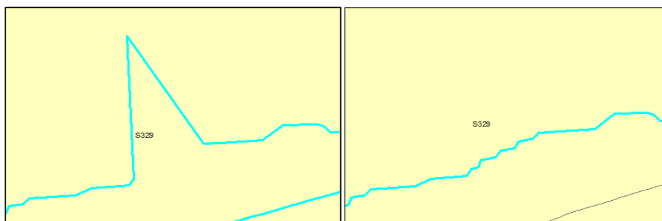
Figure 4.4: Example showing feature snapping without (left) and with (right) PRIME2
