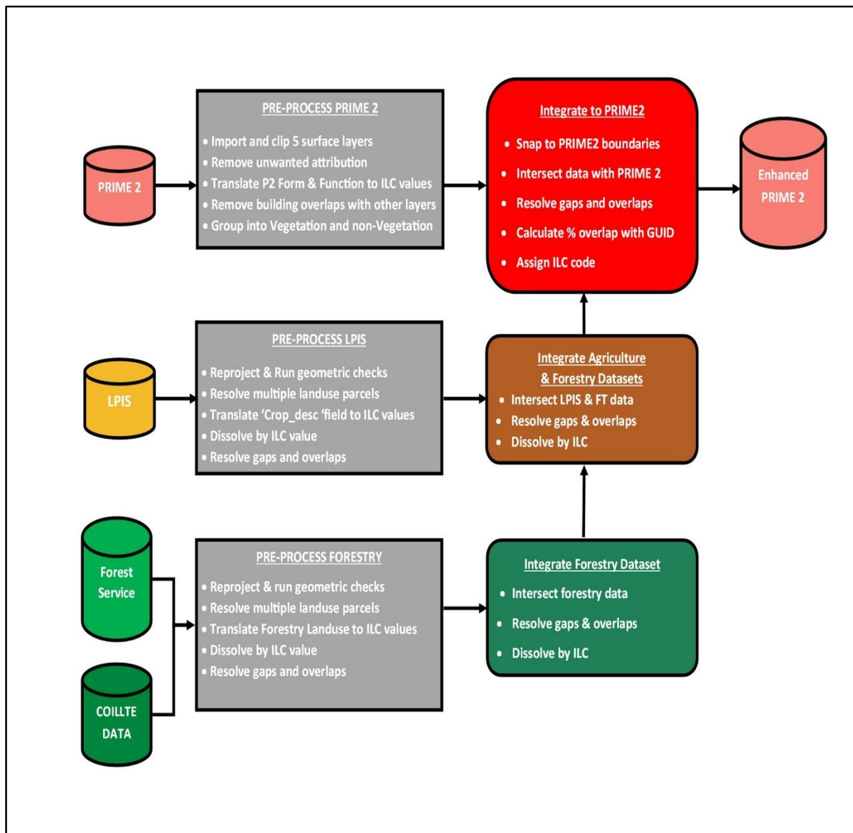
Figure 4.1: Pre-processing core vector data integration workflow
