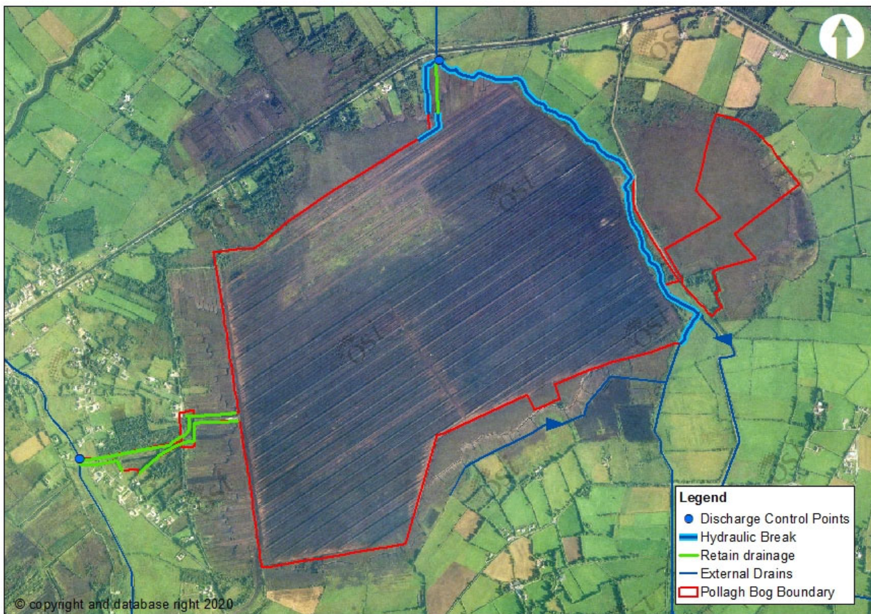
Figure 5.1 Key drainage features for Pollagh Bog
