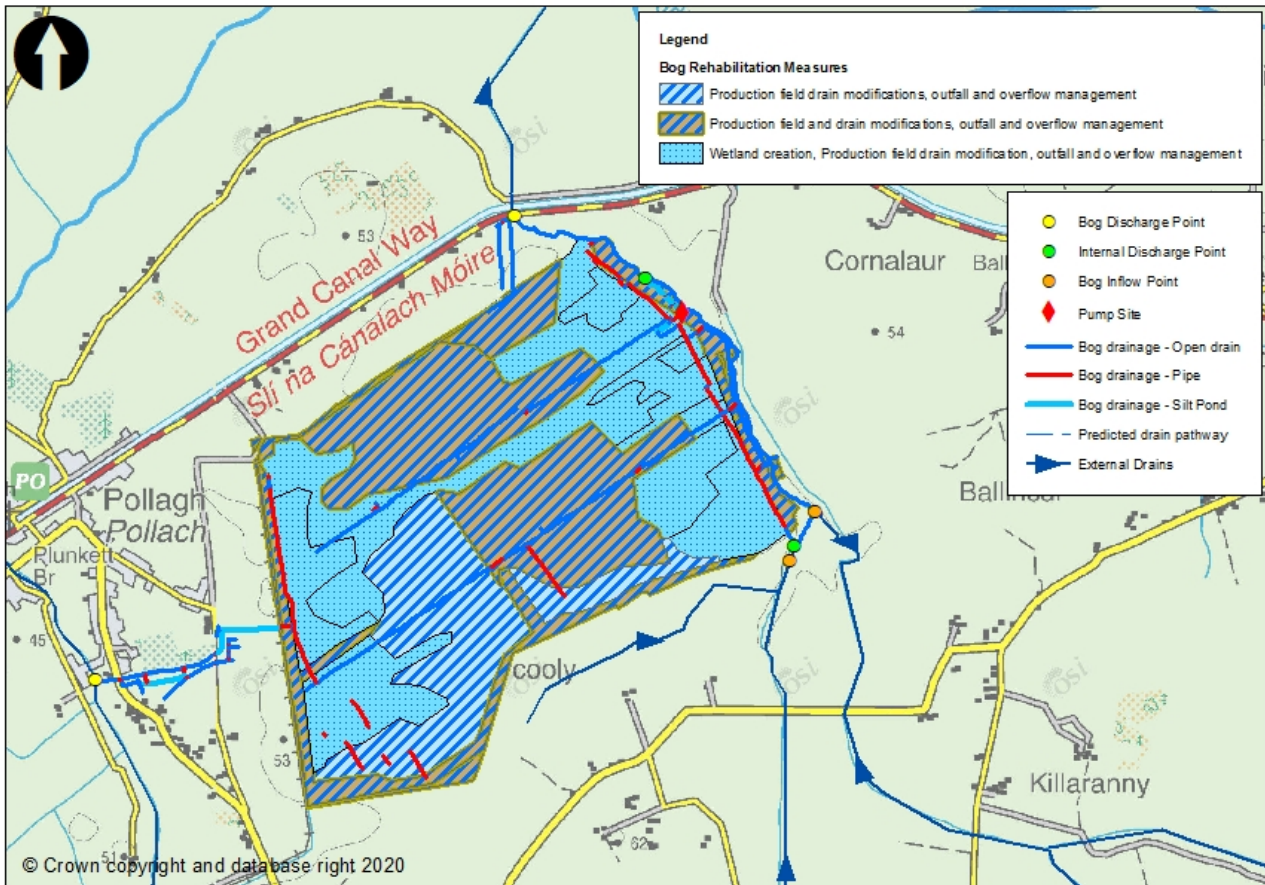
Figure 3.1 Pollagh Bog Rehabilitation Plan
