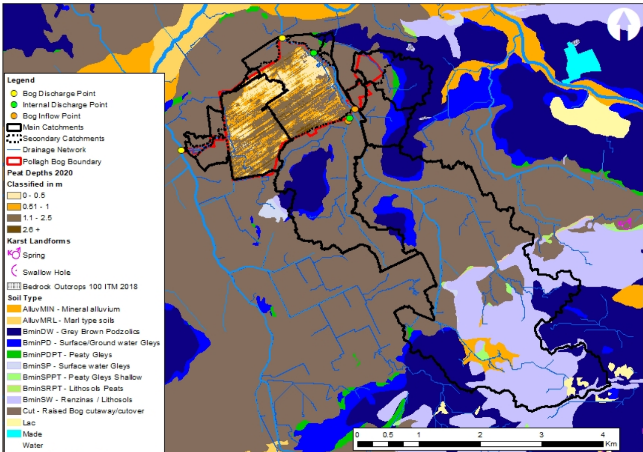
Figure 2.3 Hydrogeological and Soil Characteristics of Pollagh Bog
