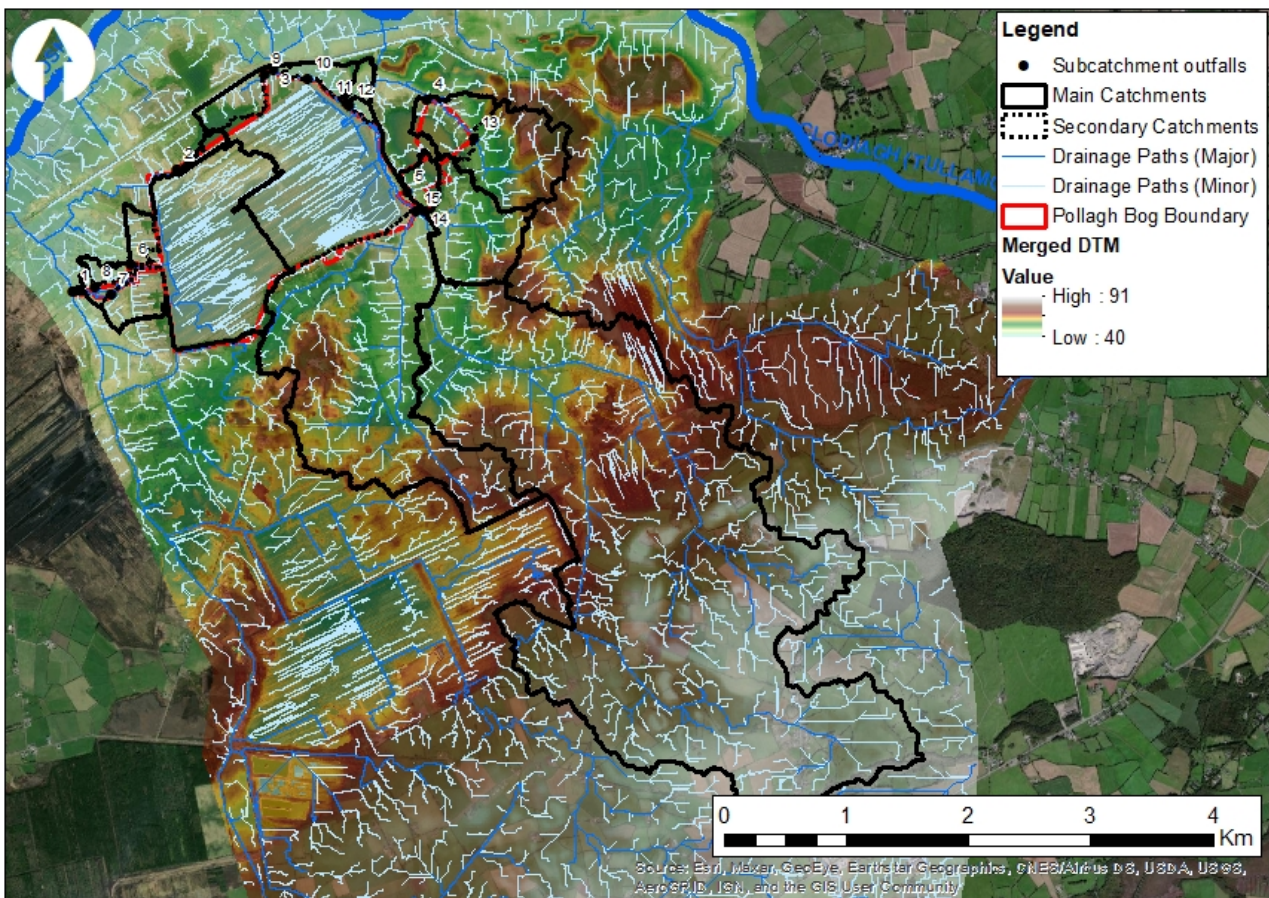
Figure 2.2 Drainage Networks and Sub-Catchments Draining Pollagh Bog
