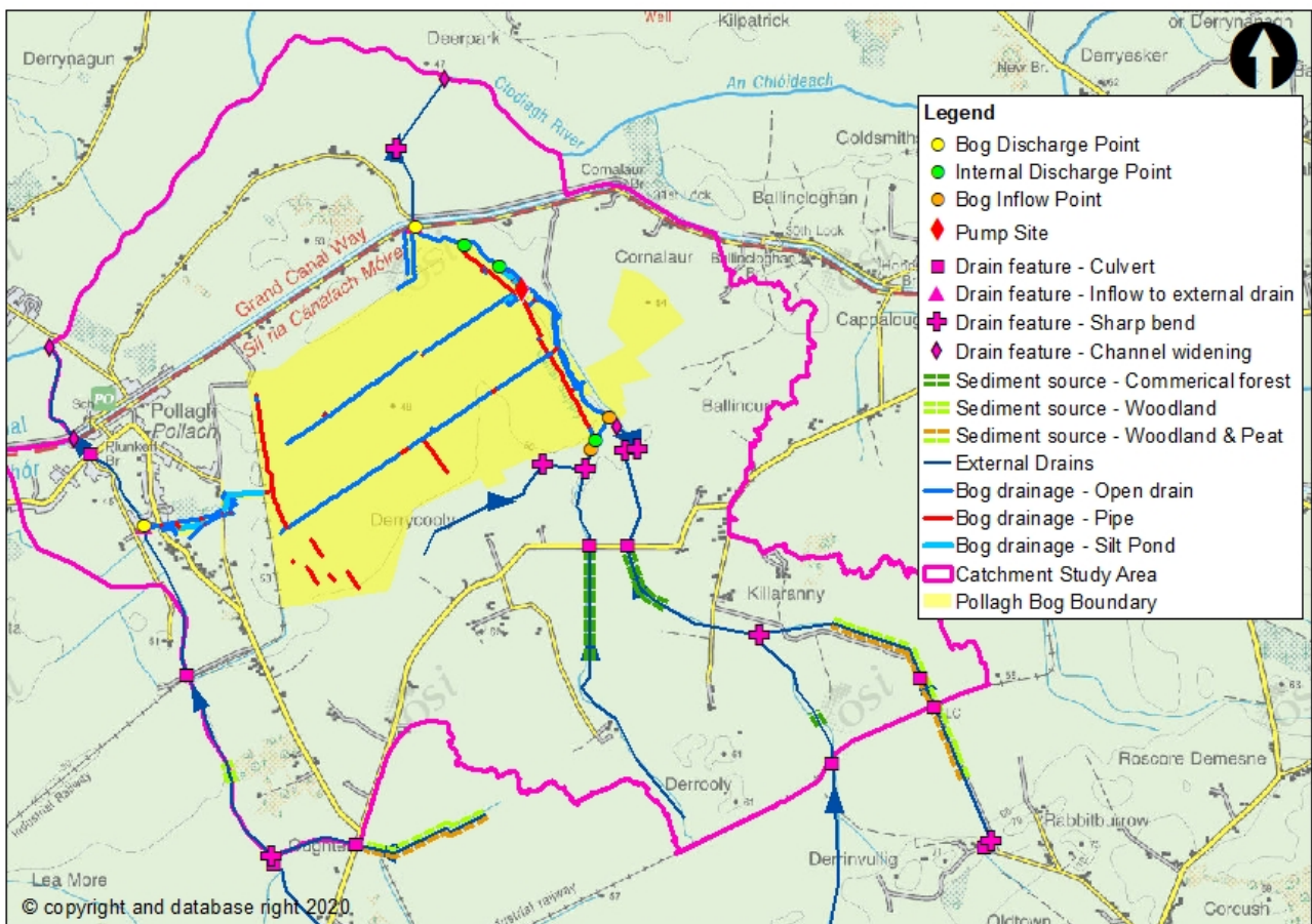
Figure 2.4 Morphological and Hydraulic Characteristics of Pollagh Bog and environs
