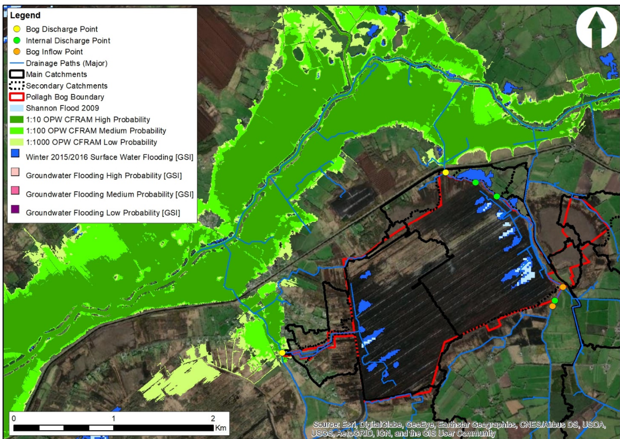
Figure 2.6 Flood Risk at Pollagh Bog
