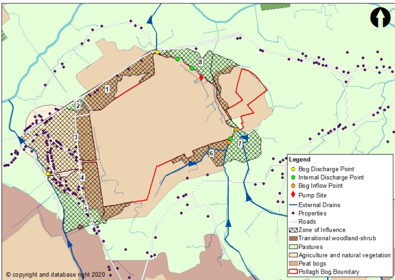
Figure 3.4 Pollagh Bog Rehabilitation Plan – Assets at risk
