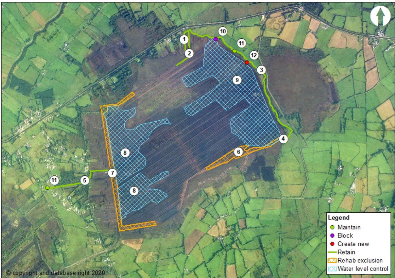
Figure 5.3 DMP measures for Pollagh Bog
