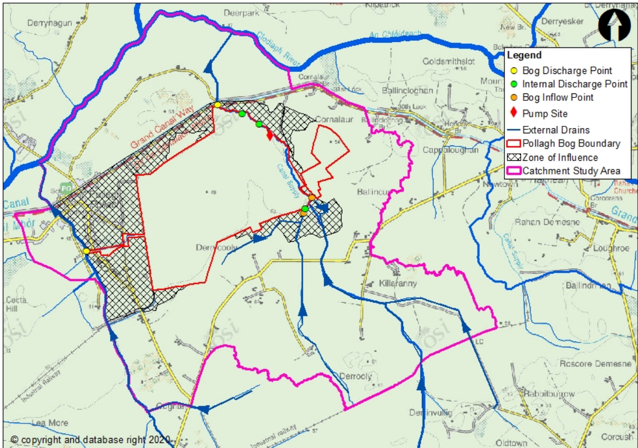
Figure 3.2 Pollagh Bog Rehabilitation Plan – Zone of influence
