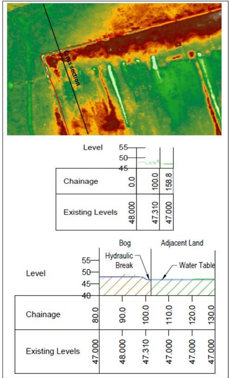
Figure 3-3 Conditions affecting water table
