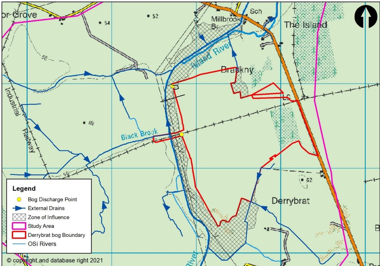
Figure 3-1 Derrybrat Bog Rehabilitation Plan – Zone of Influence
