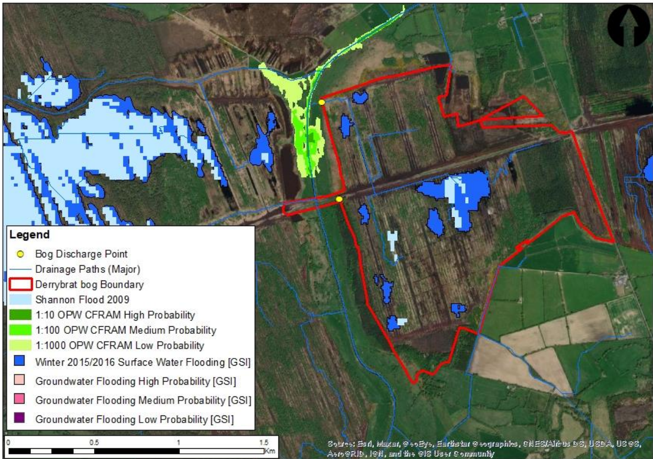
Figure 2-5 Flood Risk at Derrybrat Bog
