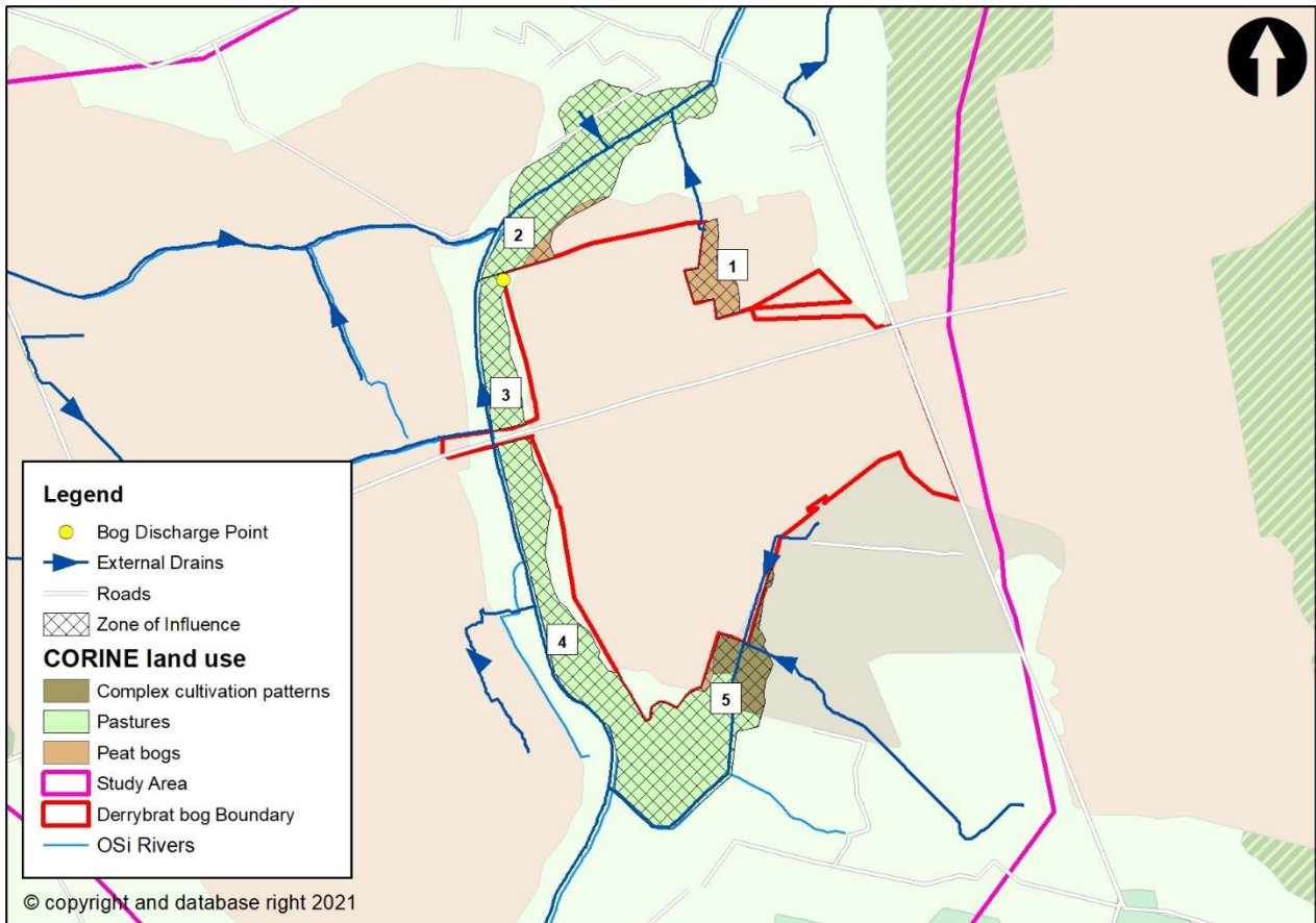
Figure 3-5 Derrybrat Bog Rehabilitation Plan – Assets At Risk
