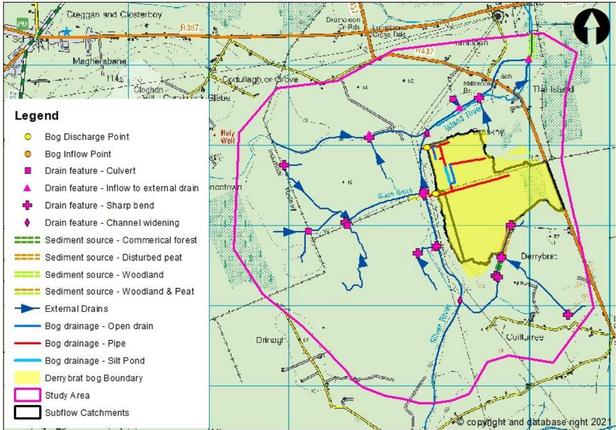
Figure 2-3 Morphological and Hydraulic Characteristics of Derrybrat Bog and environs
