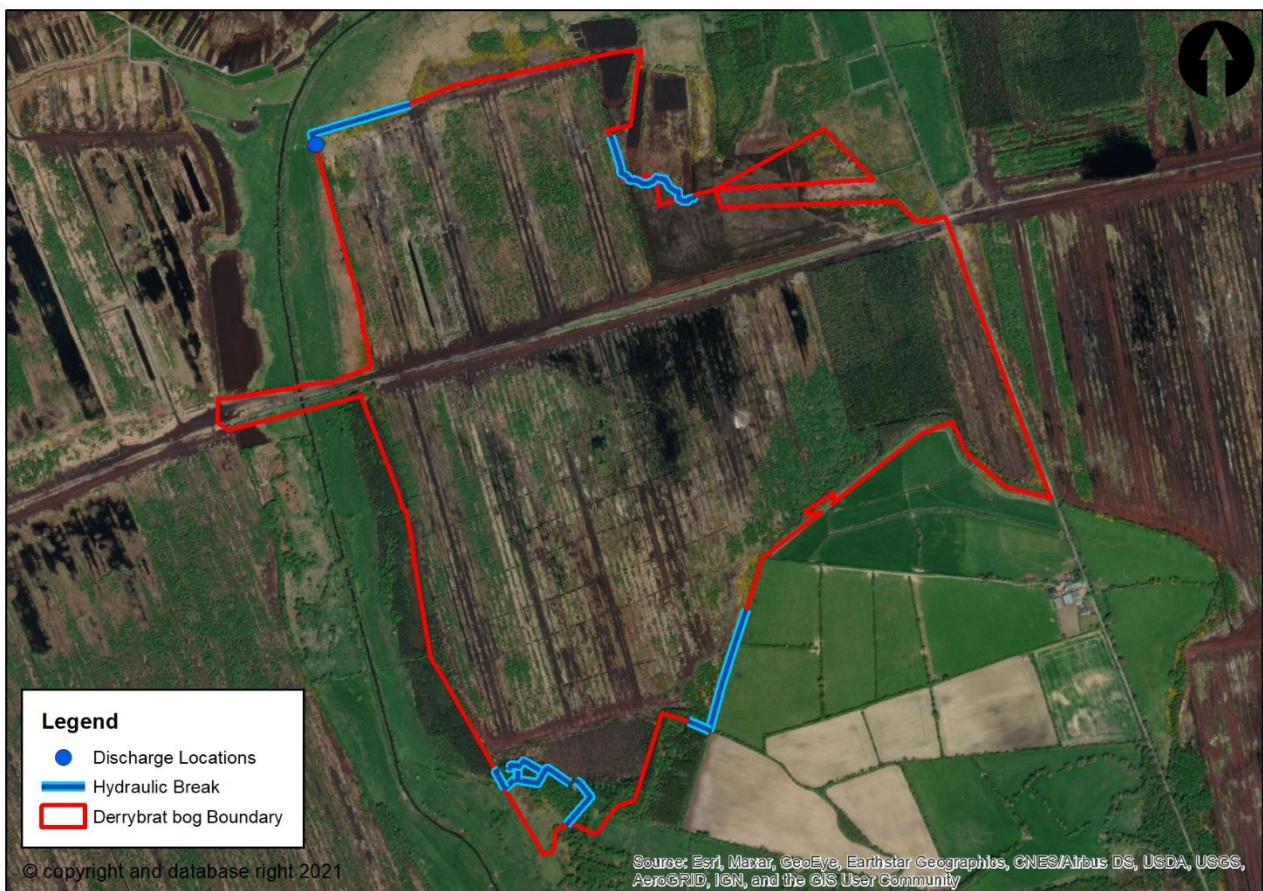
Figure 5-1 Key drainage features for Derrybrat Bog
