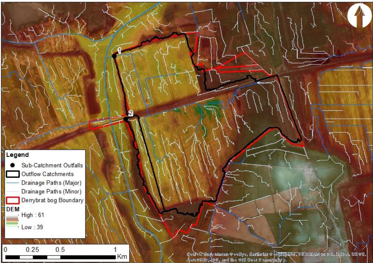
Figure 2-2 Drainage Networks and Sub-Catchments Draining Derrybrat Bog
