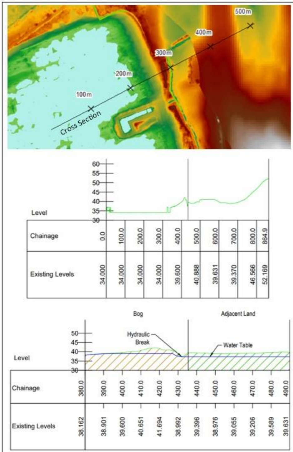
Figure 3-3 Conditions affecting water table
