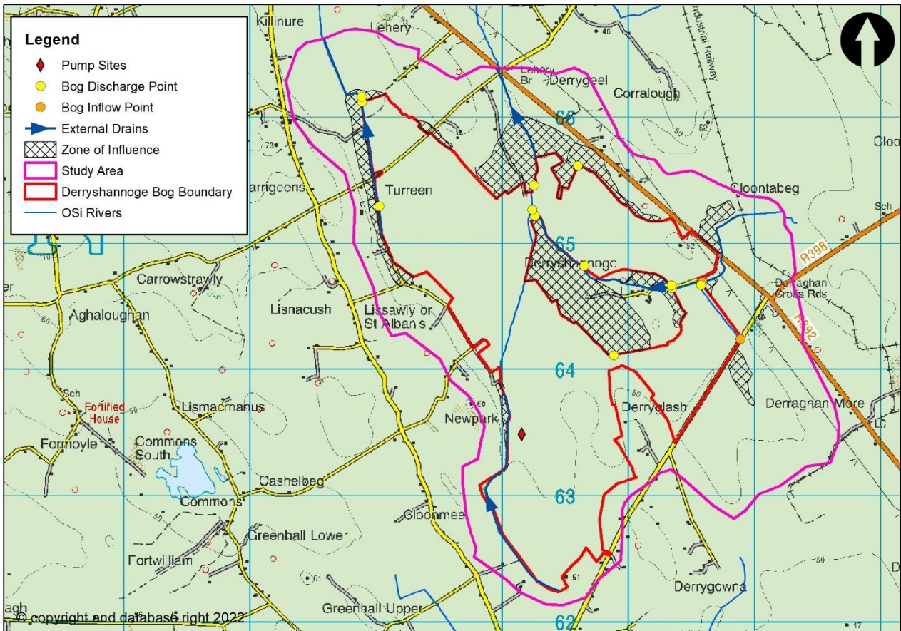
Figure 3-2 Derryshannoge Bog Rehabilitation Plan- Zone of Influence
