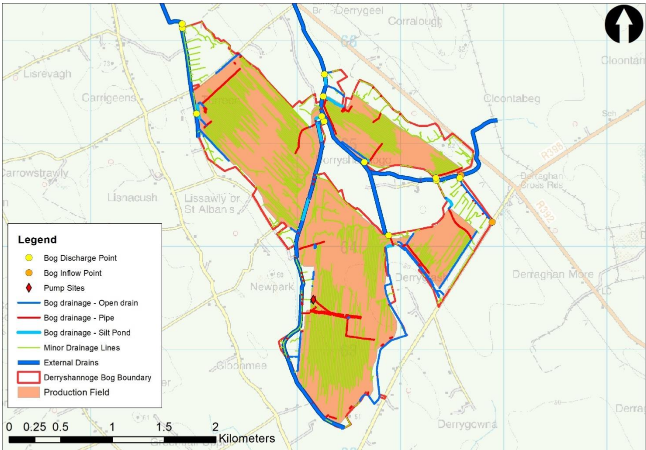
Figure E- 2: Derryshannoge production field drainage
