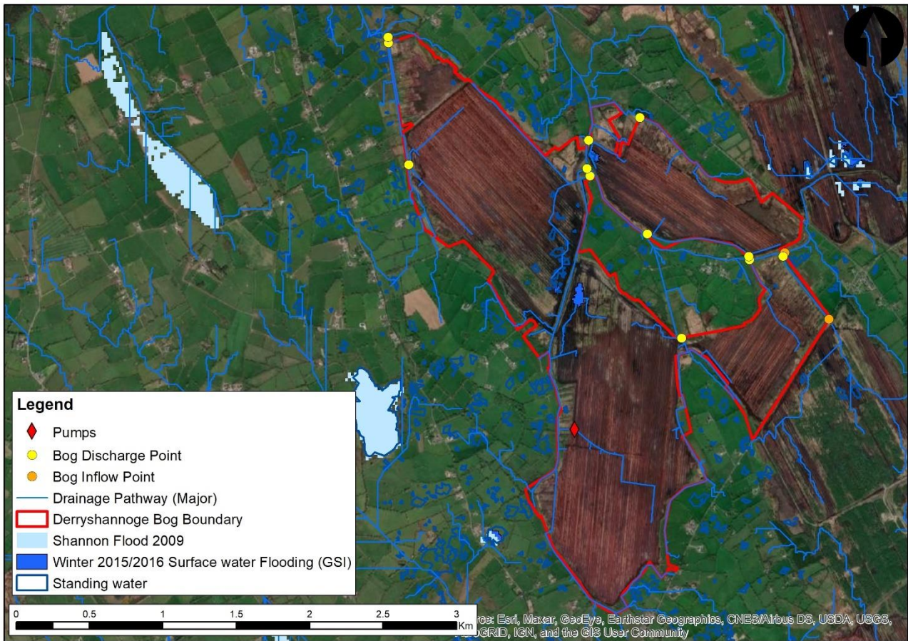
Figure 2-3 Flood Risk and Derryshannoge Bog
