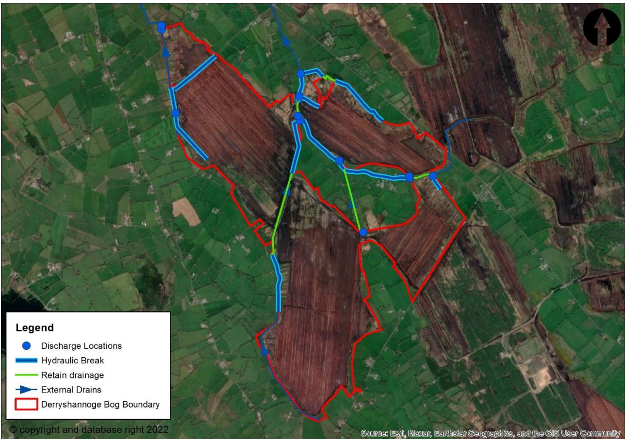
Figure 5-1 Key drainage features for Derryshannoge Bog
