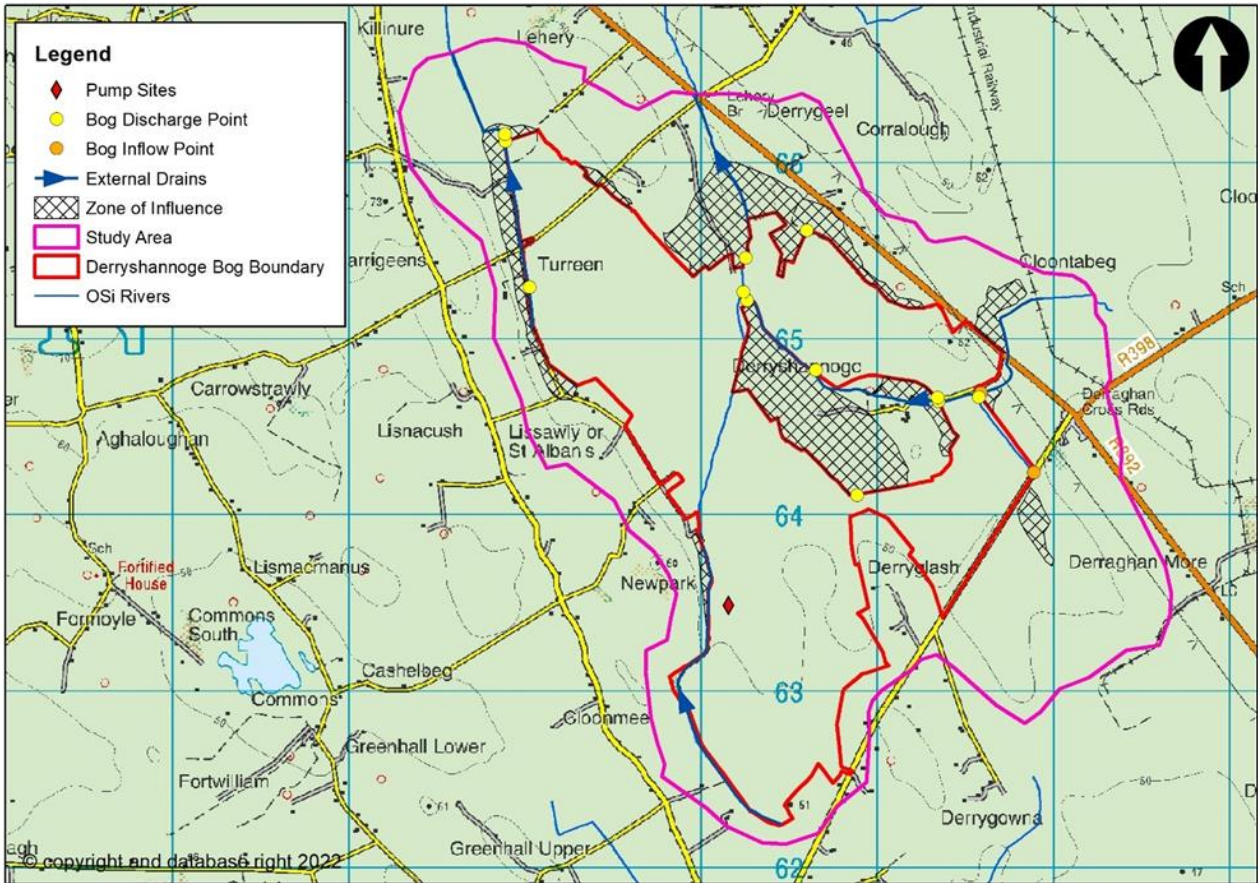
Figure E- 3: Derryshannoge Zone of influence
