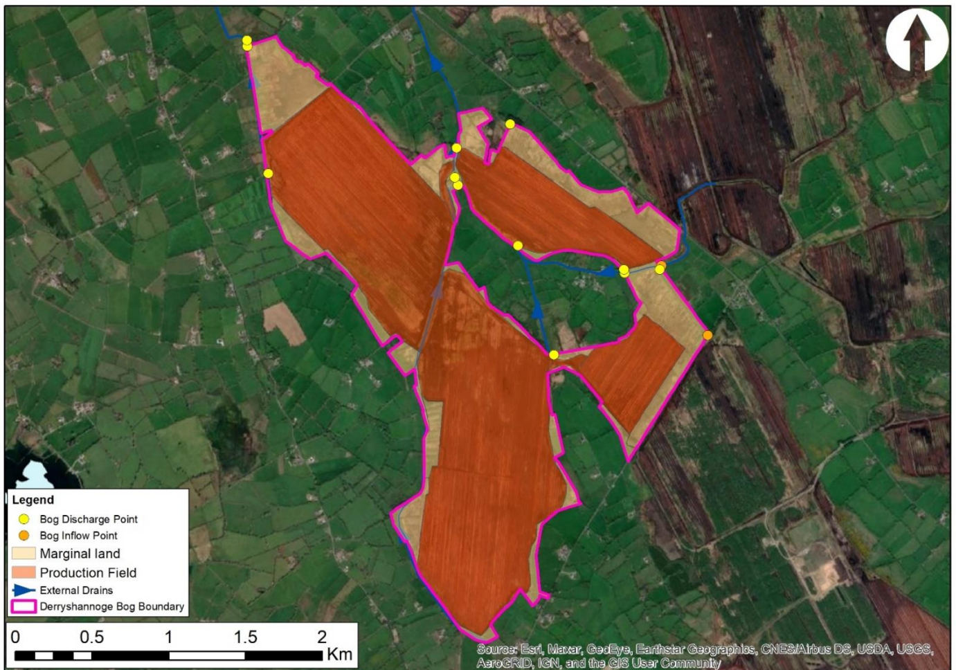
Figure 3-1- Derryshannoge bog production type
