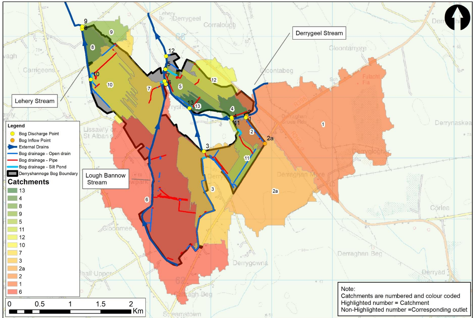
Figure 2-1 Derryshannoge Bog Drainage Network and Sub-Catchments
