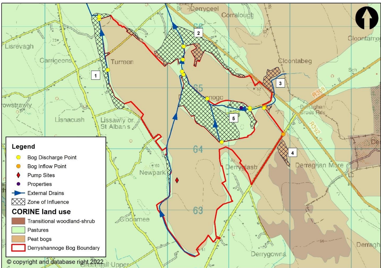
Figure 3-6 Derryshannoge Bog Rehabilitation Plan- Assets at risk
