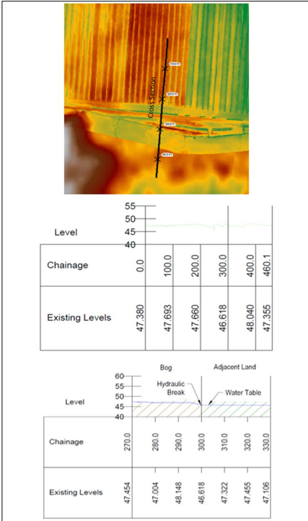
Figure 3-4 Conditions affecting water table
