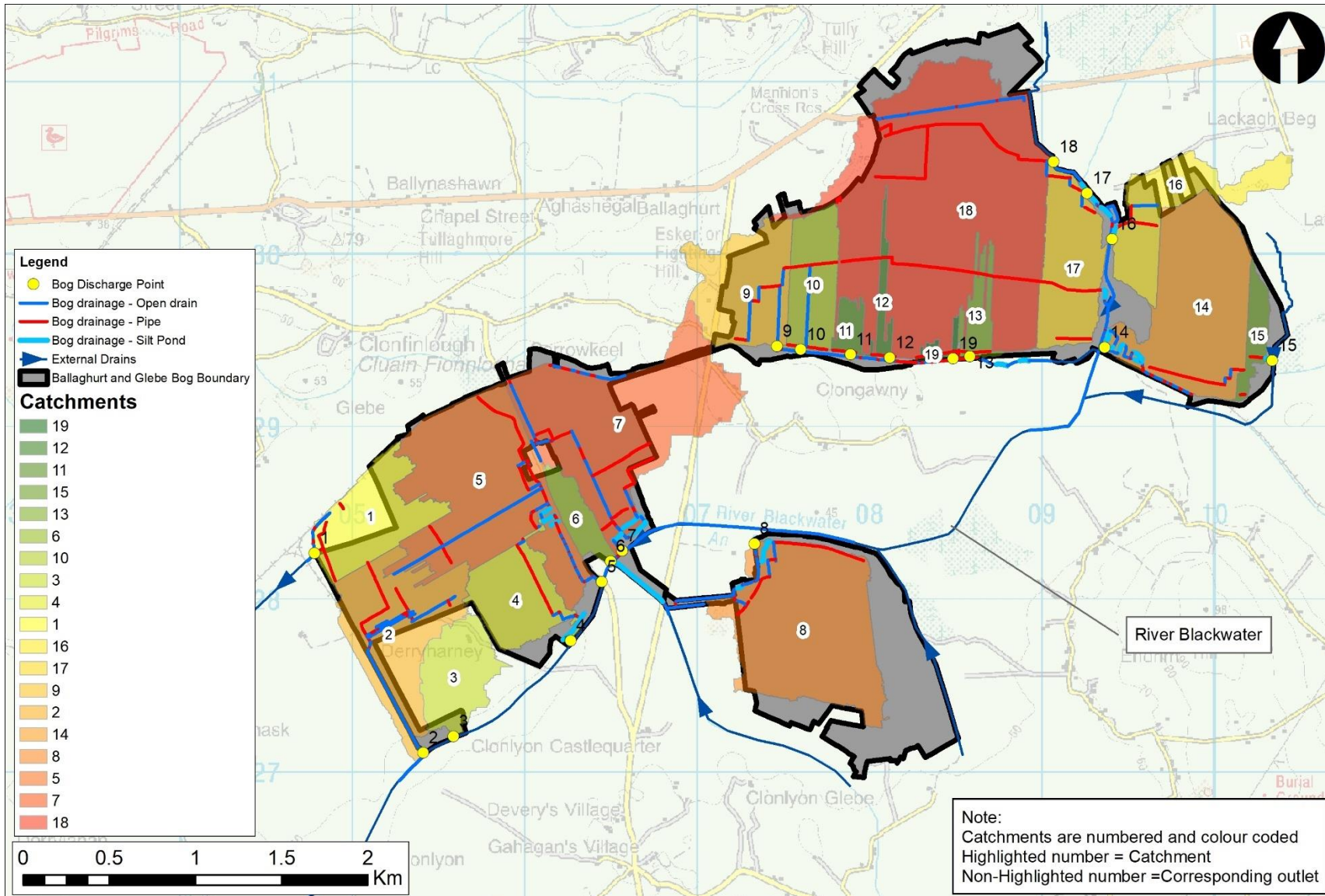
Figure 2-1 Ballaghurt and Glebe Bog Drainage Network and Sub-Catchments
