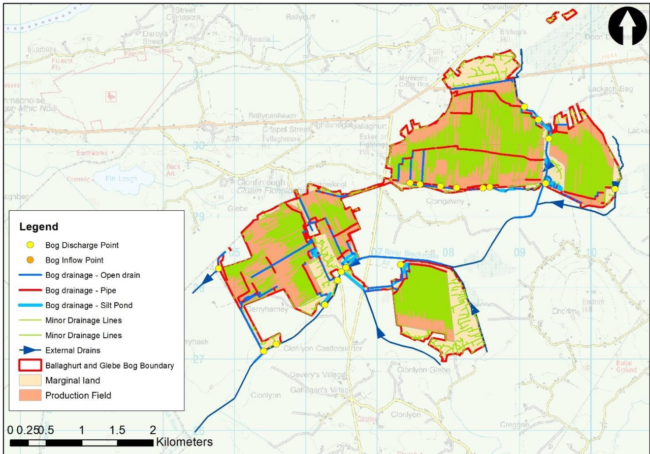
Figure E- 2: Ballaghurt and Glebe production field drainage
