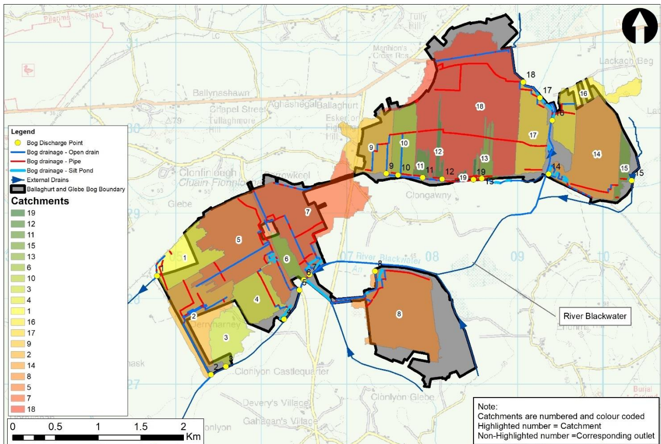
Figure E- 1: Ballaghurt and Glebe drainage catchments
