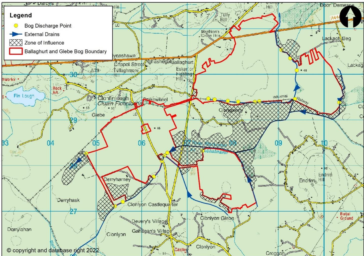
Figure E- 3: Ballaghurt and Glebe Zone of influence
