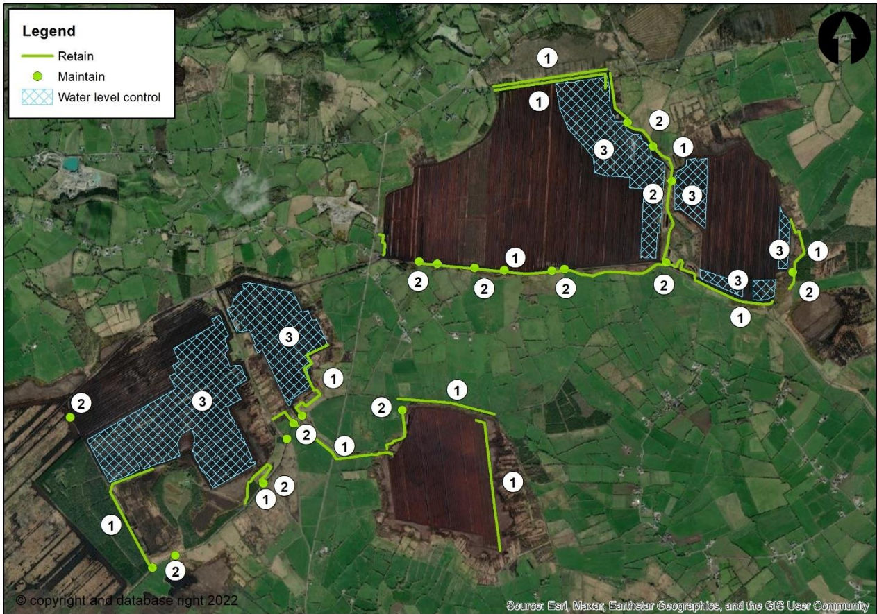
Figure 5-2 DMP measures for Ballaghurt and Glebe Bog
