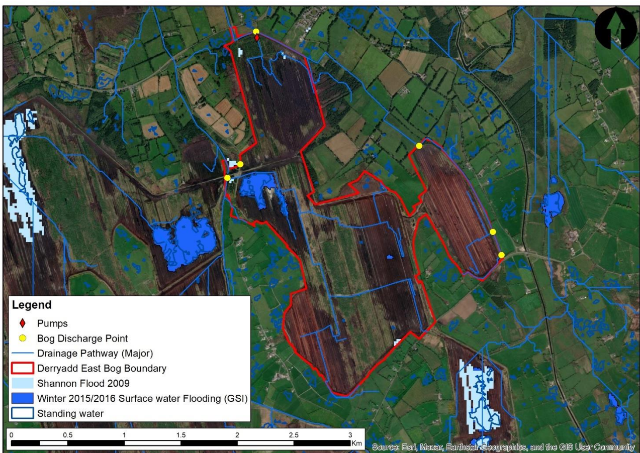
Figure 2-3 Flood Risk and Derryadd East Bog
