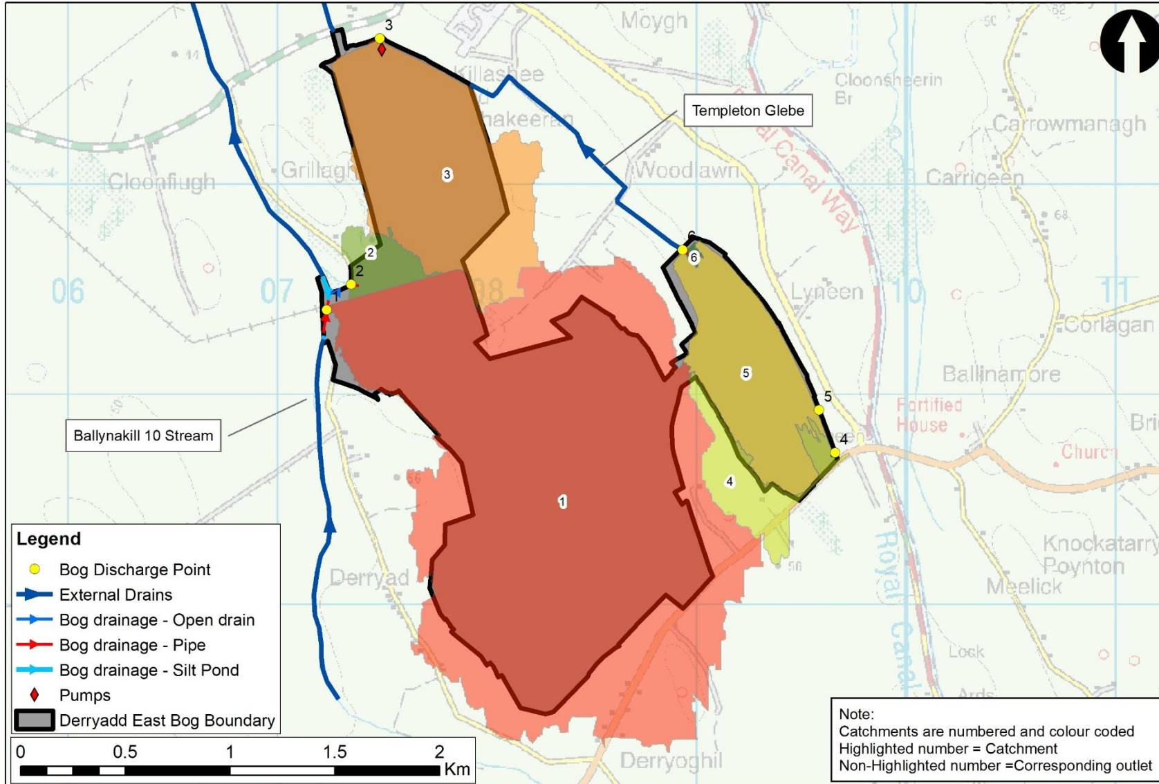
Figure 2-1 Derryadd East Bog Drainage Network and Sub-Catchments
