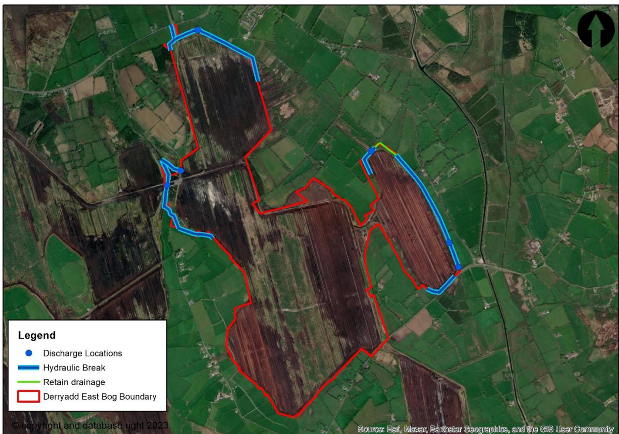
Figure 5-1 Key drainage features for Derryadd East Bog
