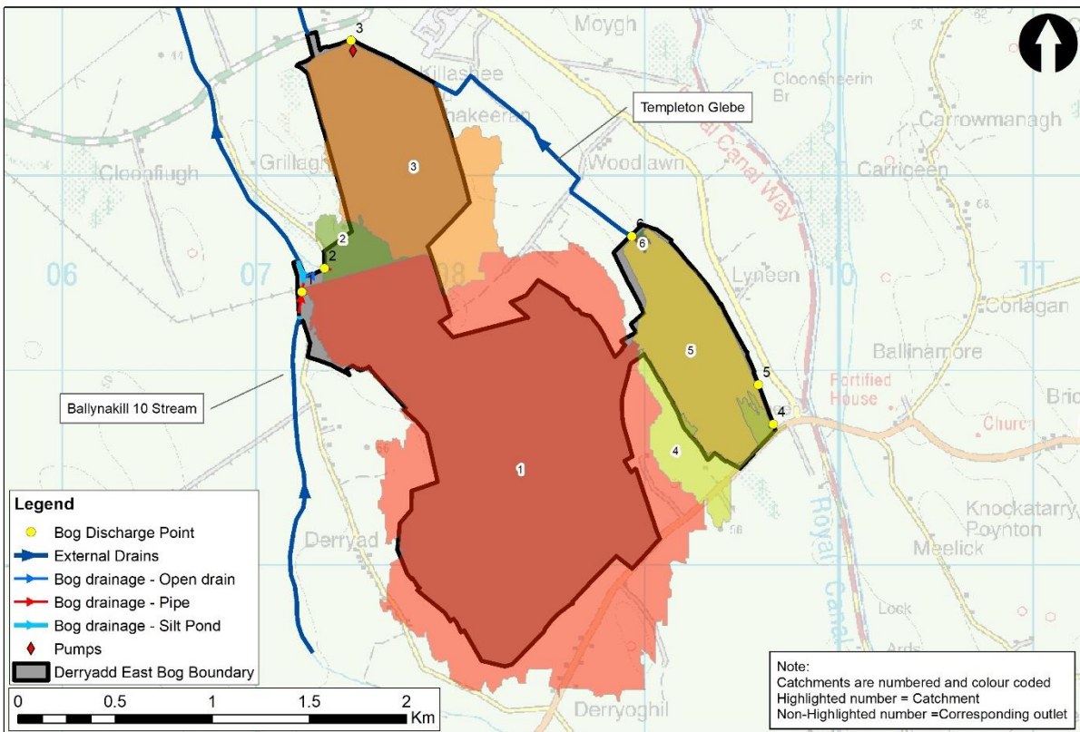
Figure E- 1: Derryadd East drainage catchments
