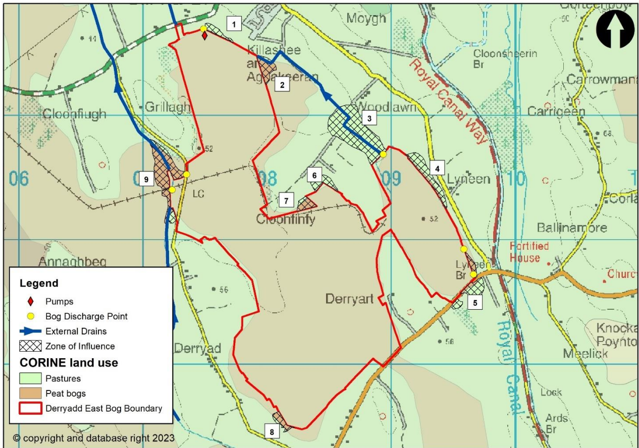
Figure 3-6 Derryadd East Bog Rehabilitation Plan- Assets at risk
