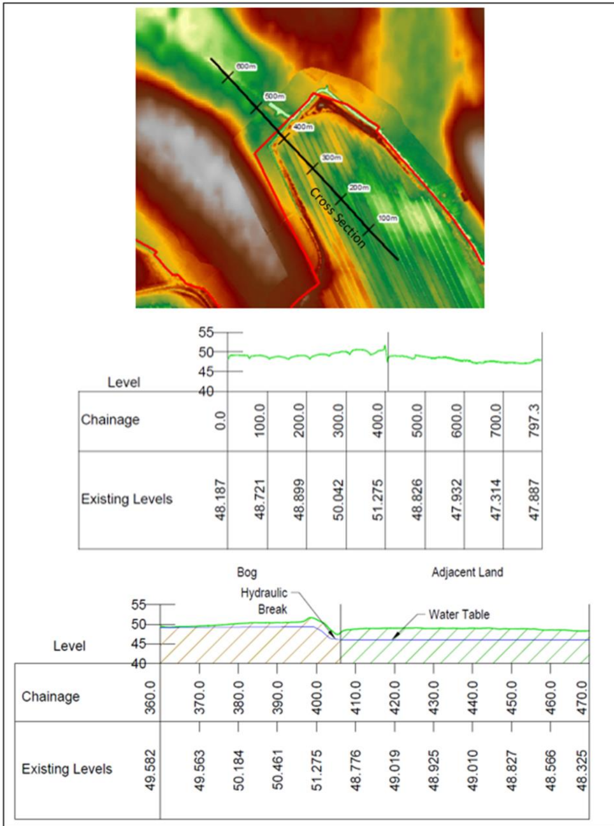
Figure 3-4 Conditions affecting water table- Cross-section of Derryadd East Bog
